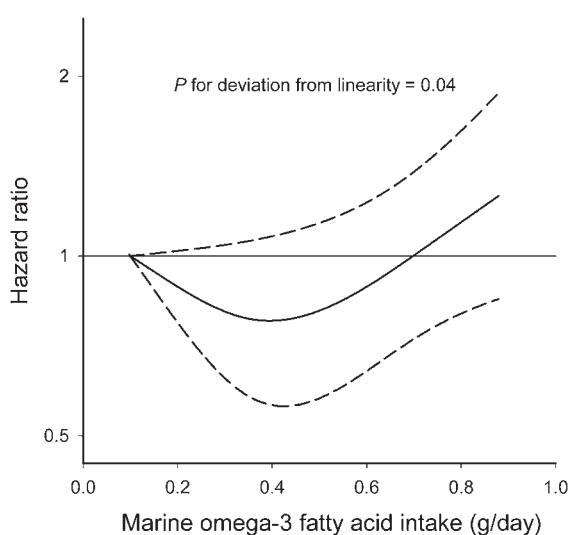
Figure 1 The solid line represents hazard ratio and the dashed line represents the 95% confidence intervals. The curve was produced from a Cox proportional hazards model where marine omega-3 intake was modelled as a restricted cubic spline with three knots, the baseline hazard was allowed to vary by age, and the hazard ratio was adjusted for body mass index, physical activity, energy, alcohol, fibre, sodium, and red or processed meat consumption, education, family history of myocardial infarction at <60 years, cigarette smoking, marital status, self-reported history of hypertension, and high cholesterol.
